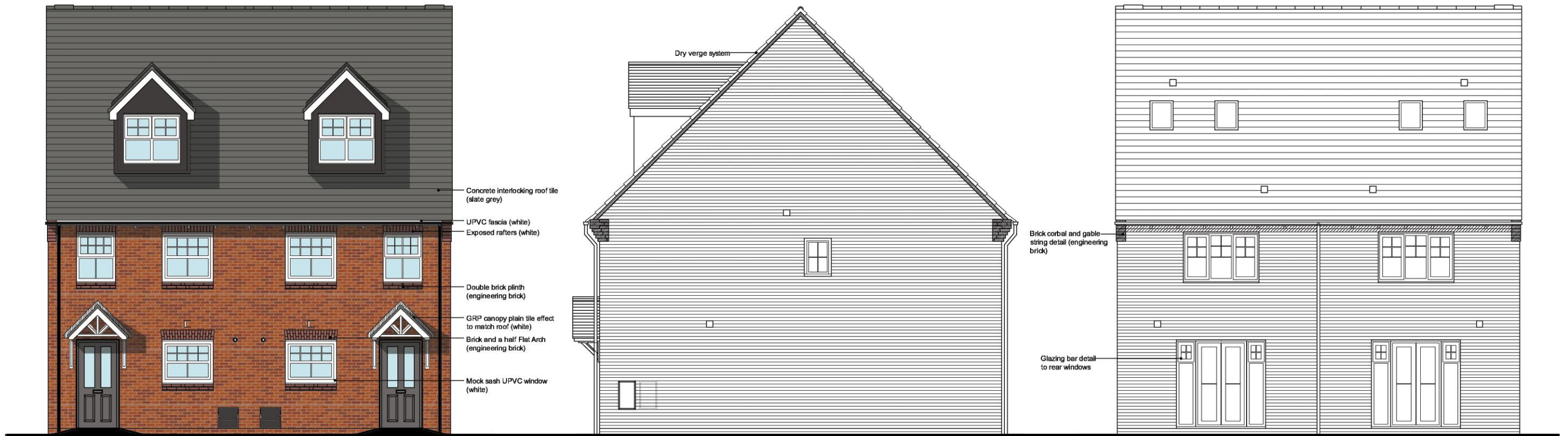
FRONT ELEVATION
